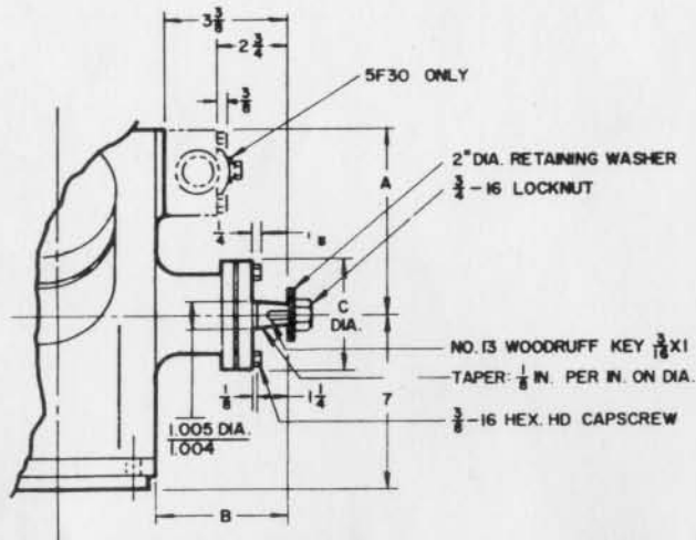
5F20 & 30 COMPRESSORS
