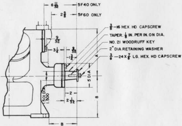
5F40 & 60 COMPRESSORS
