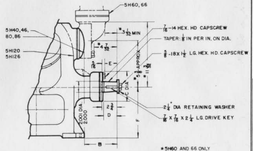
5H COMPRESSORS
