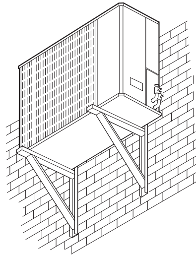
Typical Installation
