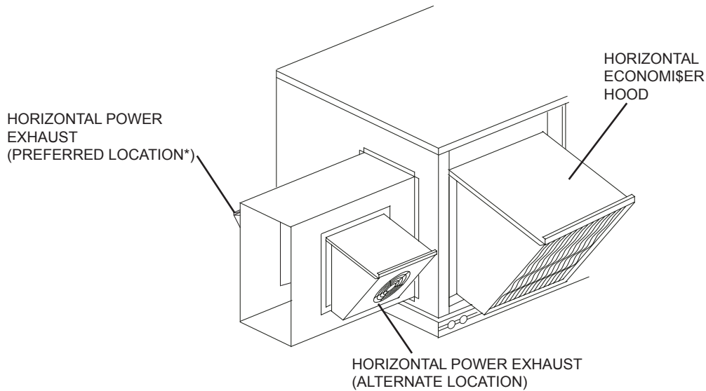
Fig. 9 - Power Exhaust Installed in Duct
