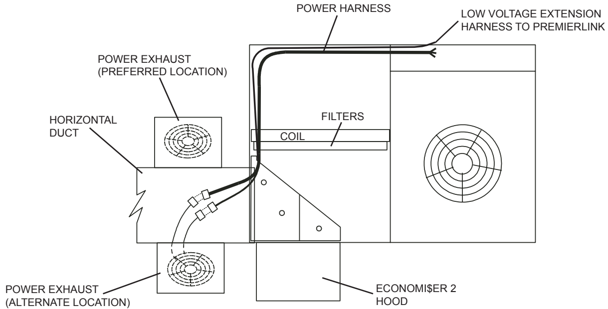
Fig. 11 - Harness Routing for EconoMiSer with PremierLink Controls (R-22 Equipped Models)
