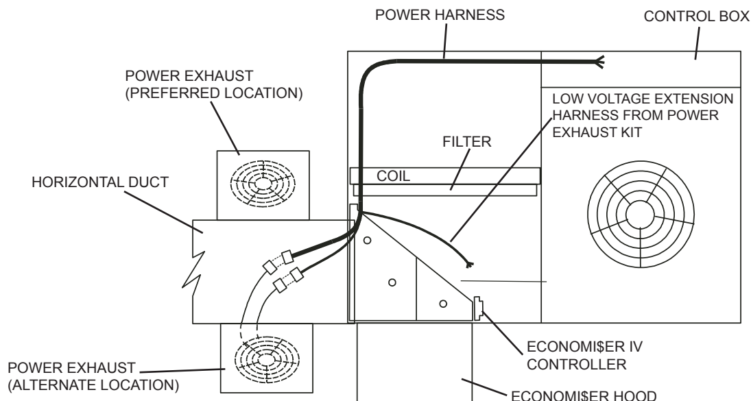
Fig. 4 - Power Exhaust Harness Routing for EconoMiSer IV and EconoMiSer X
