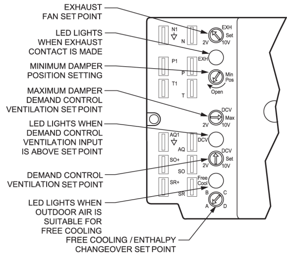
Fig. 4 - EconomiSer IV Controller Potentiometer and LED Locations
