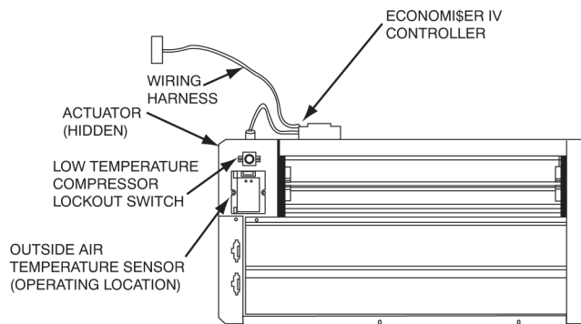
Fig. 1 - EconomiSer IV Component Locations
