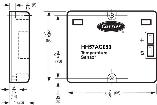
Fig. 3 - Temperature Sensor Specifications
