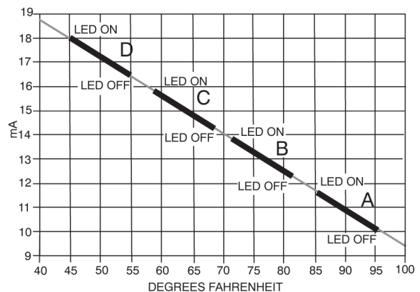
Fig. 5 - Outdoor Air Changeover Temperature
