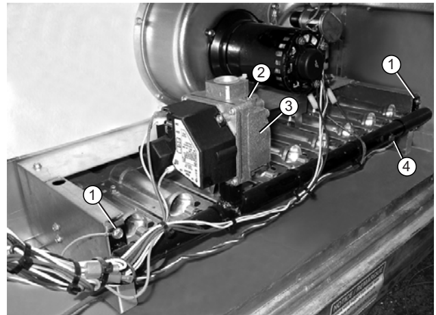
Fig. 1 - Typical Base Unit
