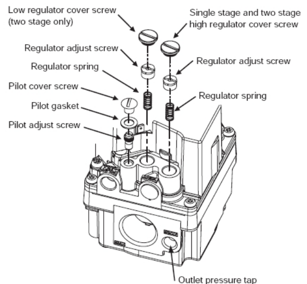
Fig. 5 - Two-Stage Spring Installation
