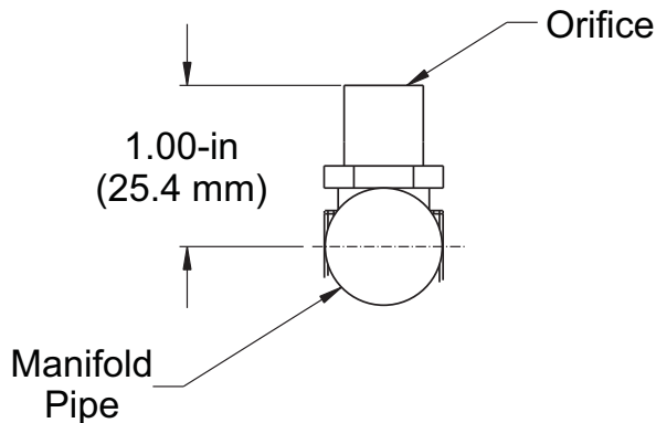
Fig. 3 - Orifice Projection
