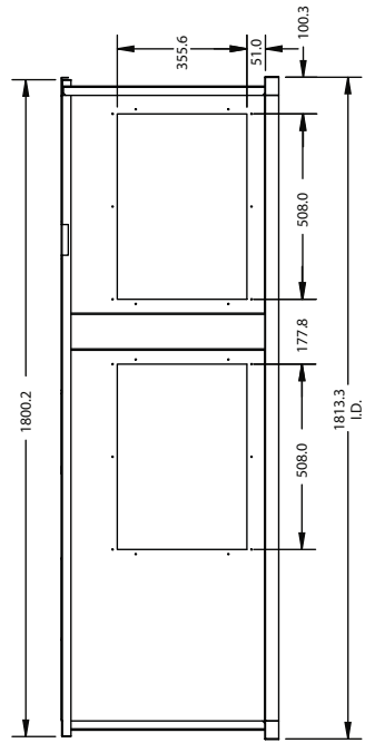
Fig. 2 - CRADCURB007A00 Horizontal Curb Adapter Assembly
