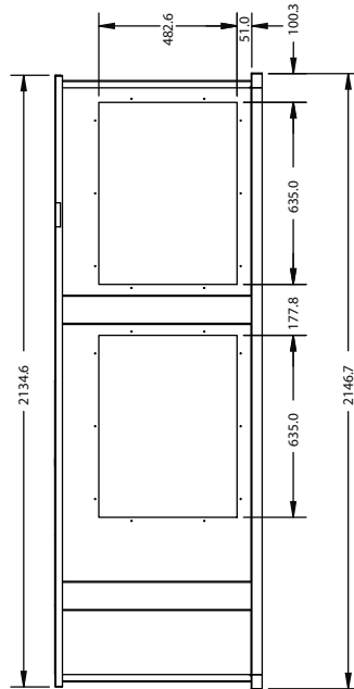
Fig. 3 - CRADCURB008A00 Horizontal Curb Adapter Assembly
