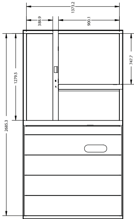
Fig. 4 - CRADCURB009A00 Horizontal Curb Adapter Assembly
