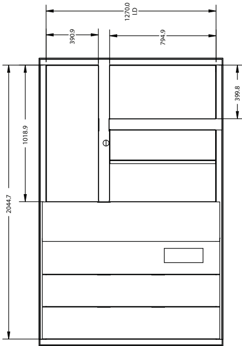
Fig. 3 - CRADCURB008A00 Horizontal Curb Adapter Assembly
