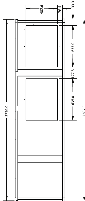
Fig. 4 - CRADCURB009A00 Horizontal Curb Adapter Assembly
